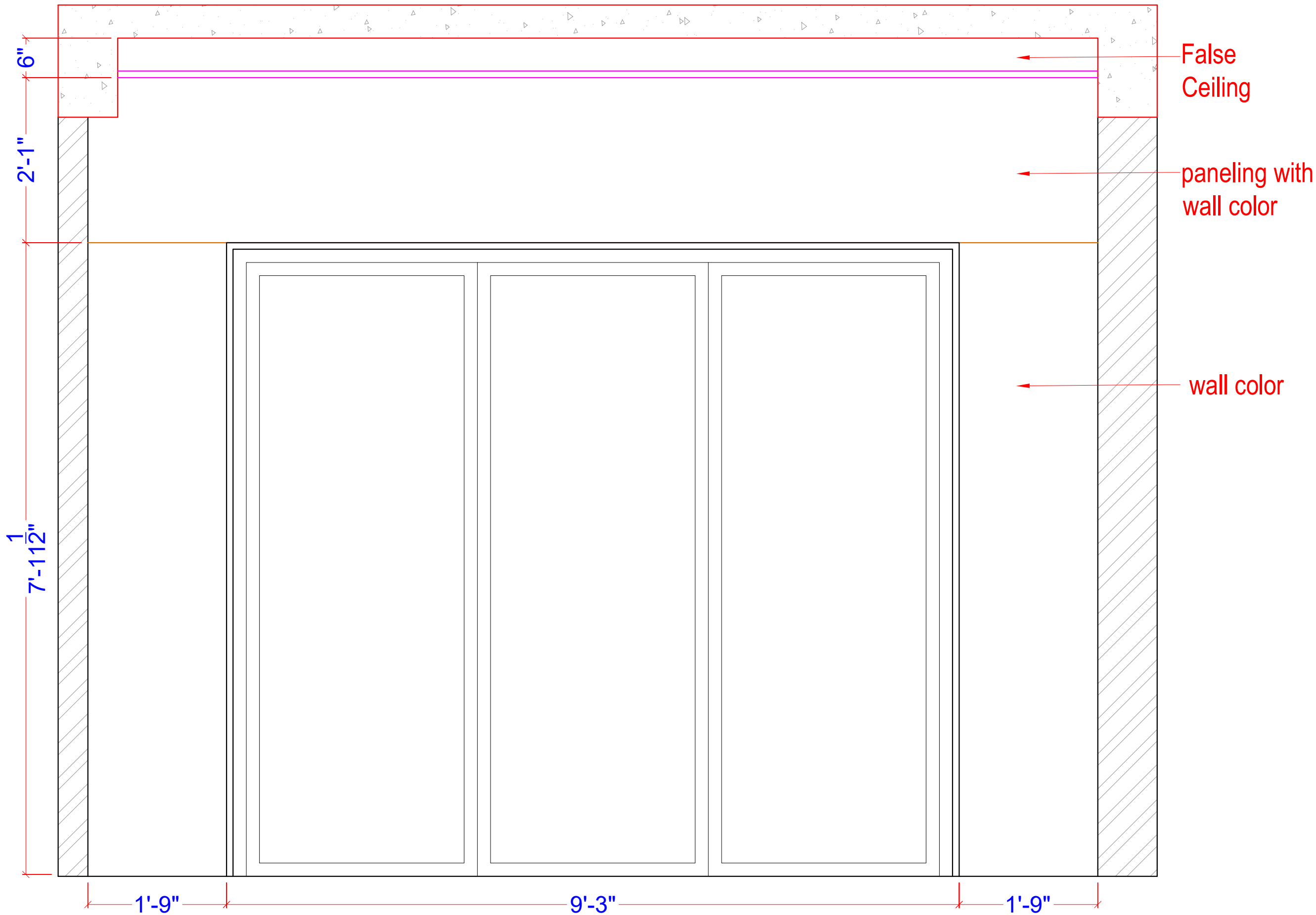
WALL ELEVATION - D
