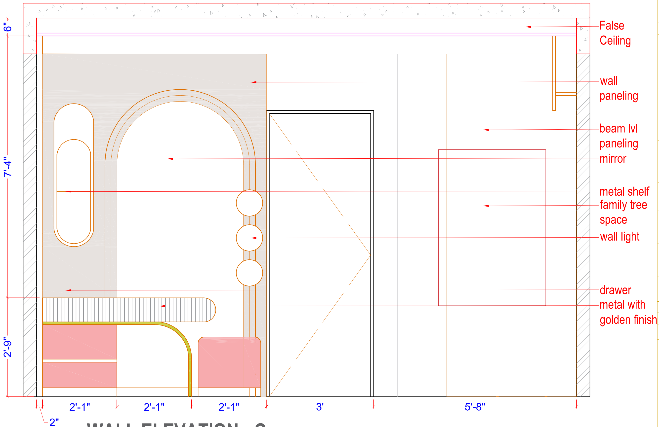
WALL ELEVATION - C
